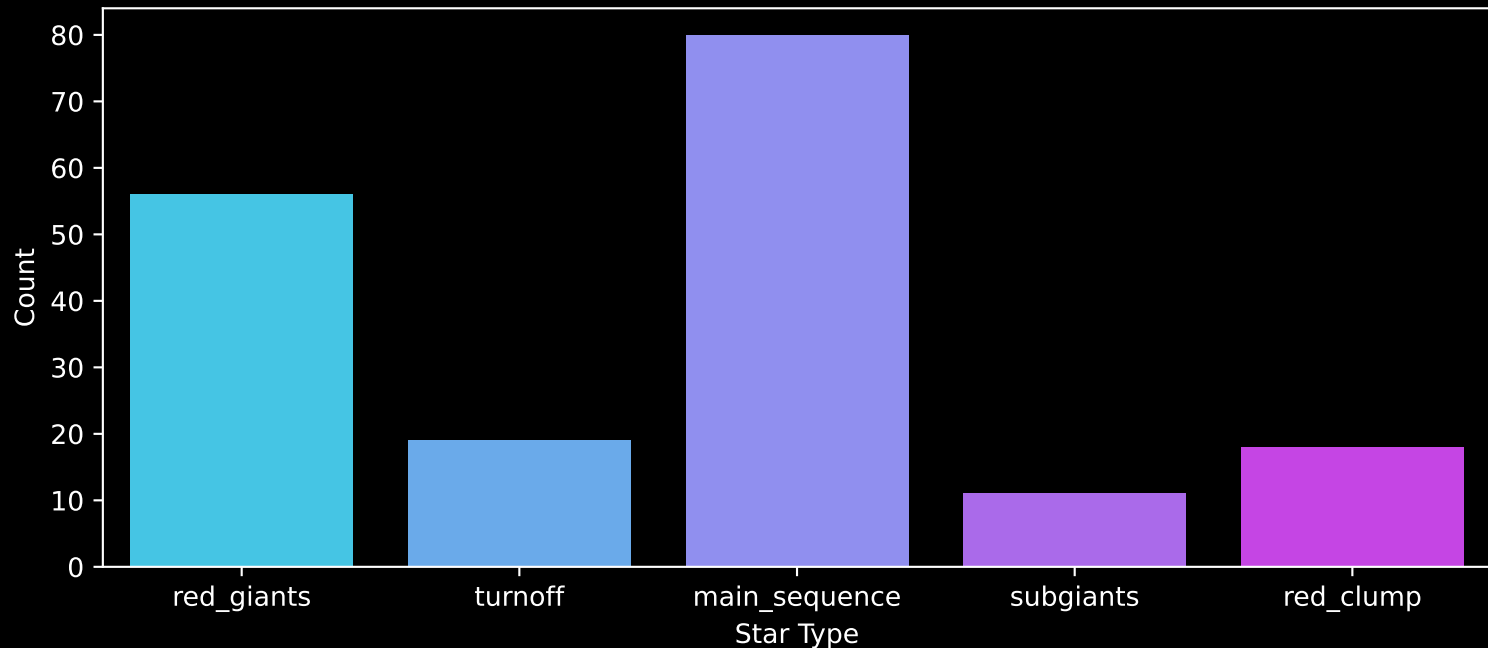
APOGEE DR17 Field: [CVZTILE_093+32_btx] Count plot of Star Type
