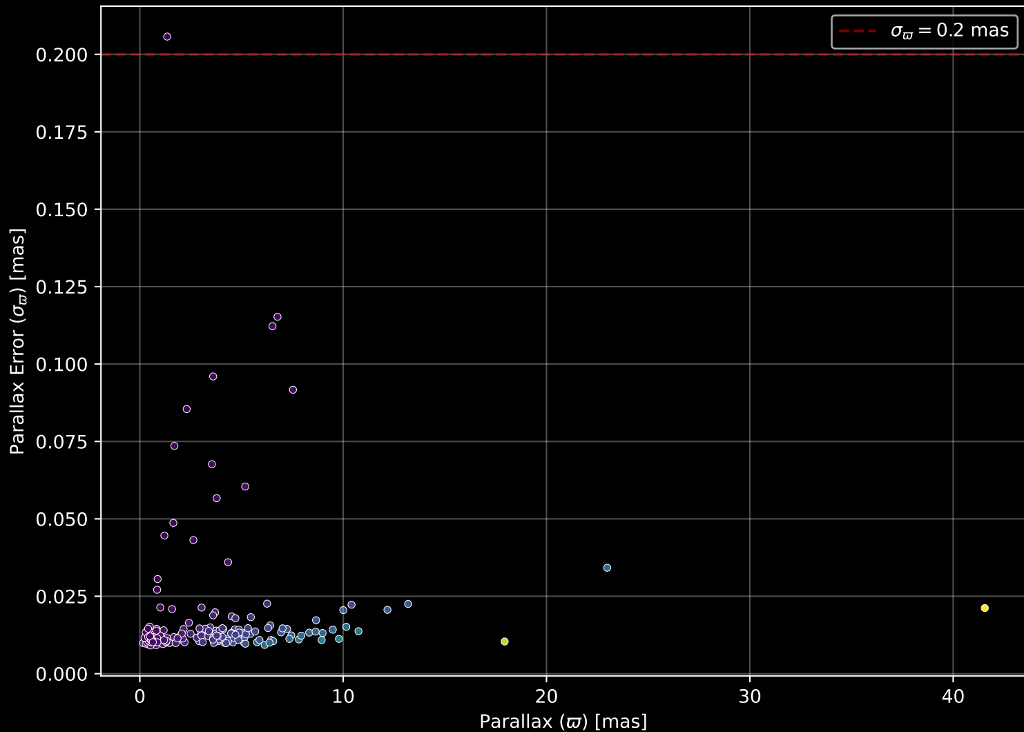
APOGEE DR17 Field: [CVZTILE_093+32_btx] Parallax Quality (n= 184)
