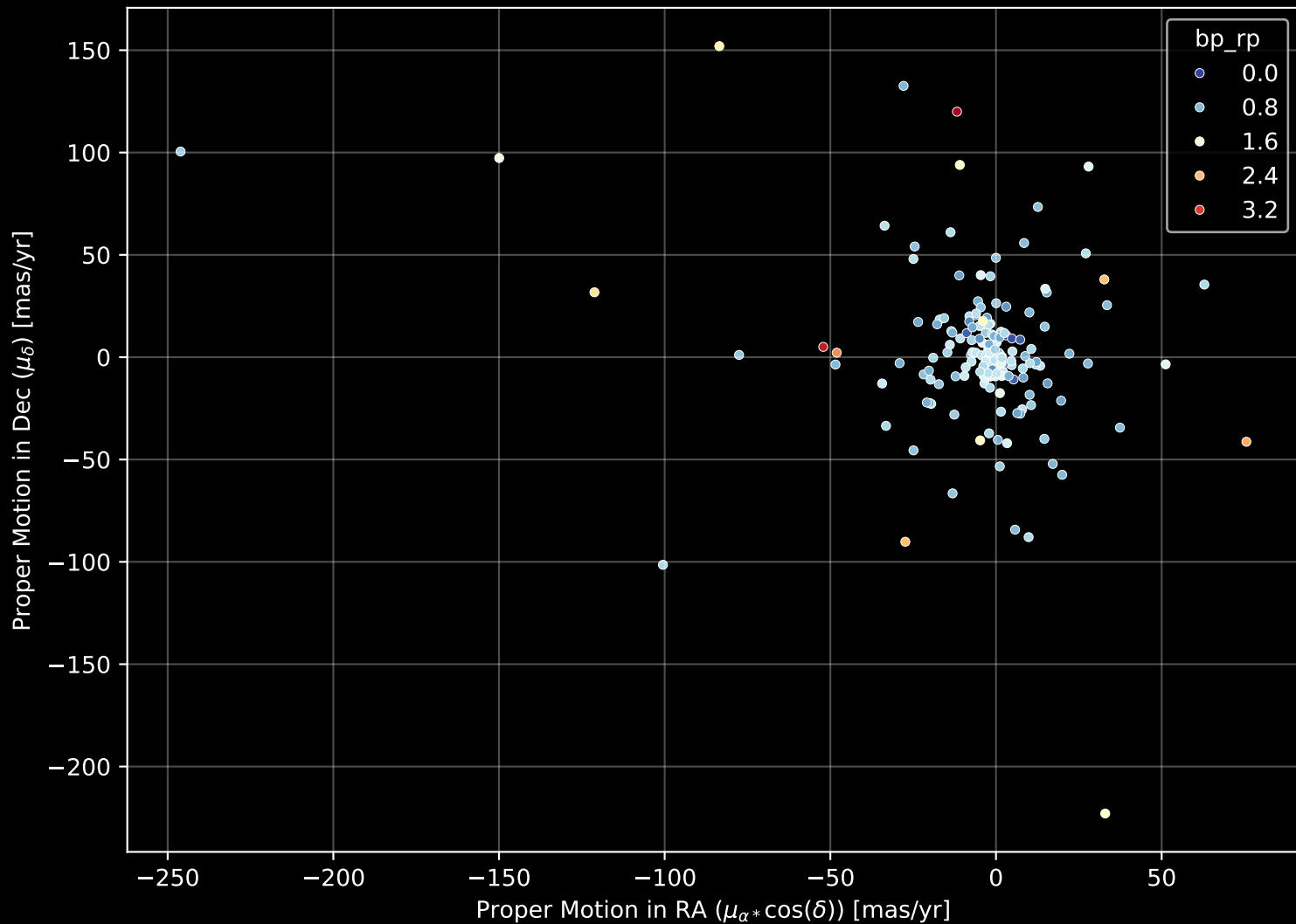
APOGEE DR17 Field: [CVZTILE_093+32_btx] Proper Motion Diagram (n= 184)
