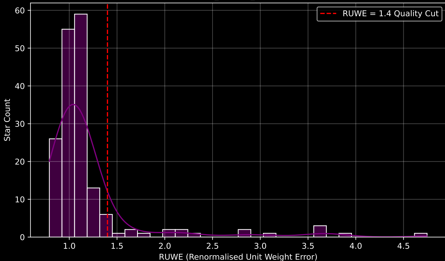
GAPOGEE DR17 Field [CVZTILE_093+32_btx] RUWE Distribution (n= 176)
