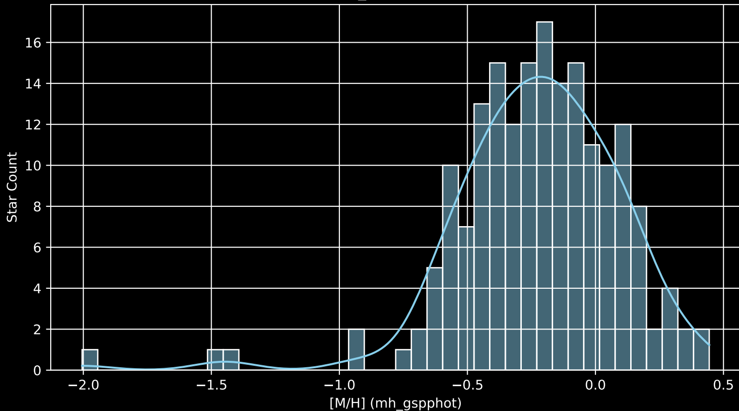
APOGEE DR17 Field: [CVZTILE_093+32_btx [M/H] (mh_gspphot) (n= 182)
